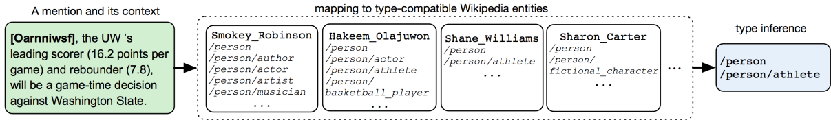
Figure 1: ZOE maps a given mention to its type-compatible entities in Wikipedia and infers a collection of types using this set of entities. While the mention “Oarnniwsf,” a football player in the U. of Washington, does not exist in Wikipedia, we ground it to other entities with approximately the same types (§3).
